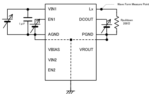
< Circuit No.5 >
