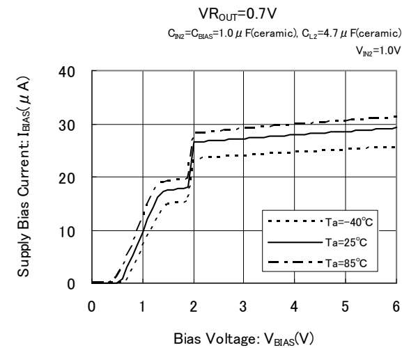
(5) Supply Bias Current vs. Bias Voltage
