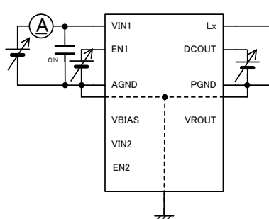
< Circuit No.9 >
