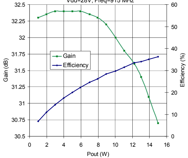
CW Gain, Efficiency vs Pout Vdd=28V, Freq=915 MHz
