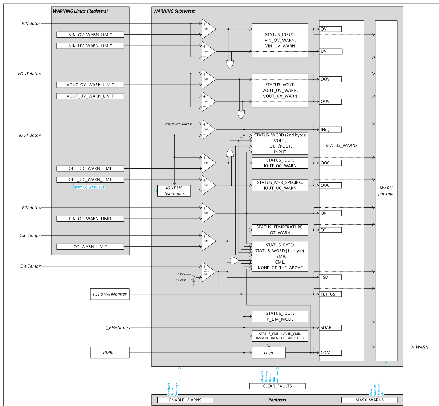
Figure 10 Warnings flow
