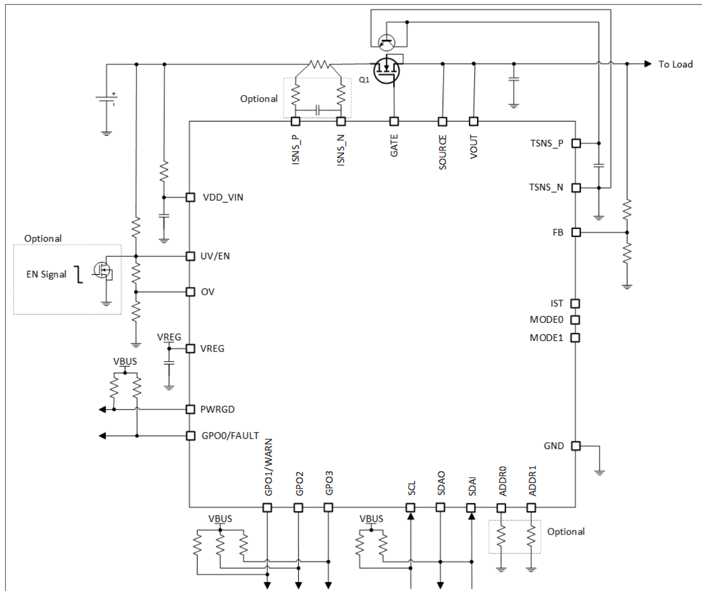
Figure 32 Fully digital mode ACM (MODE:MODE=0x0) application schematic
