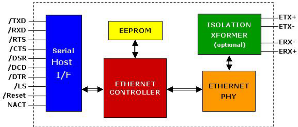
XE232NET Block Diagram
