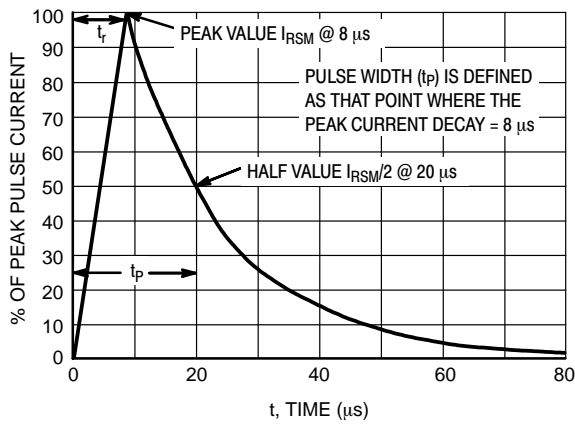
Figure 1. 8 x 20 \mu s Pulse Waveform
