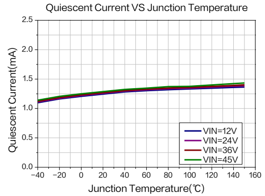
Figure13. Quiescent Current
