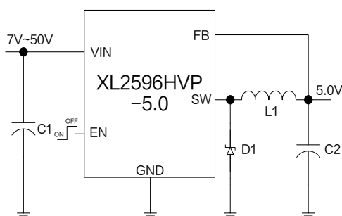
Figure1.XL2596HVP-5.0 Typical application schematic and efficiency curve
