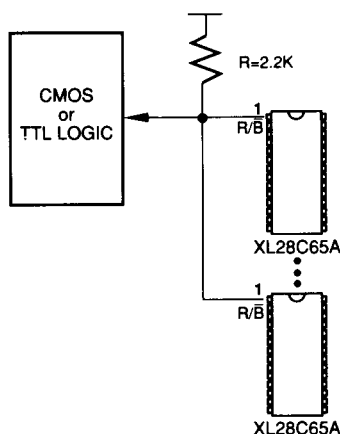
Figure 1. OR-Tied \overline{R/\overline{B}} Pins
