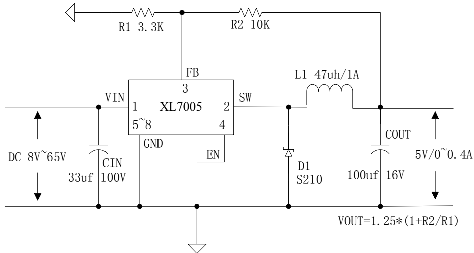
Figure7. XL7005 System Application (VIN=8V~65V, VOUT=5V)
