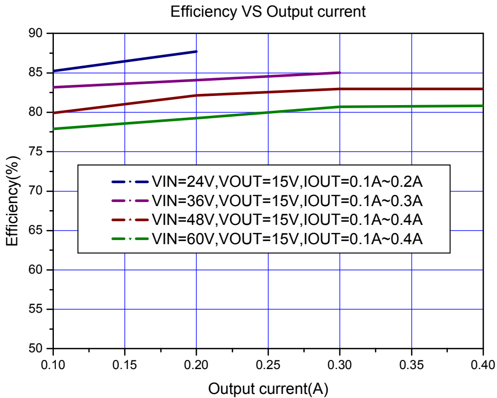
Figure6. XL7005 System Application (Efficiency VS Output Current)
