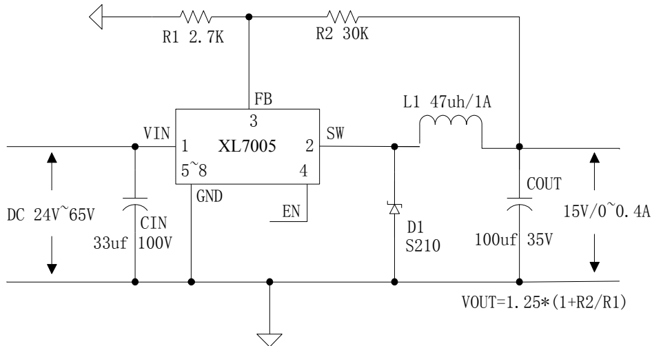
Figure5. XL7005 System Application (VIN=24V~65V, VOUT=15V)
