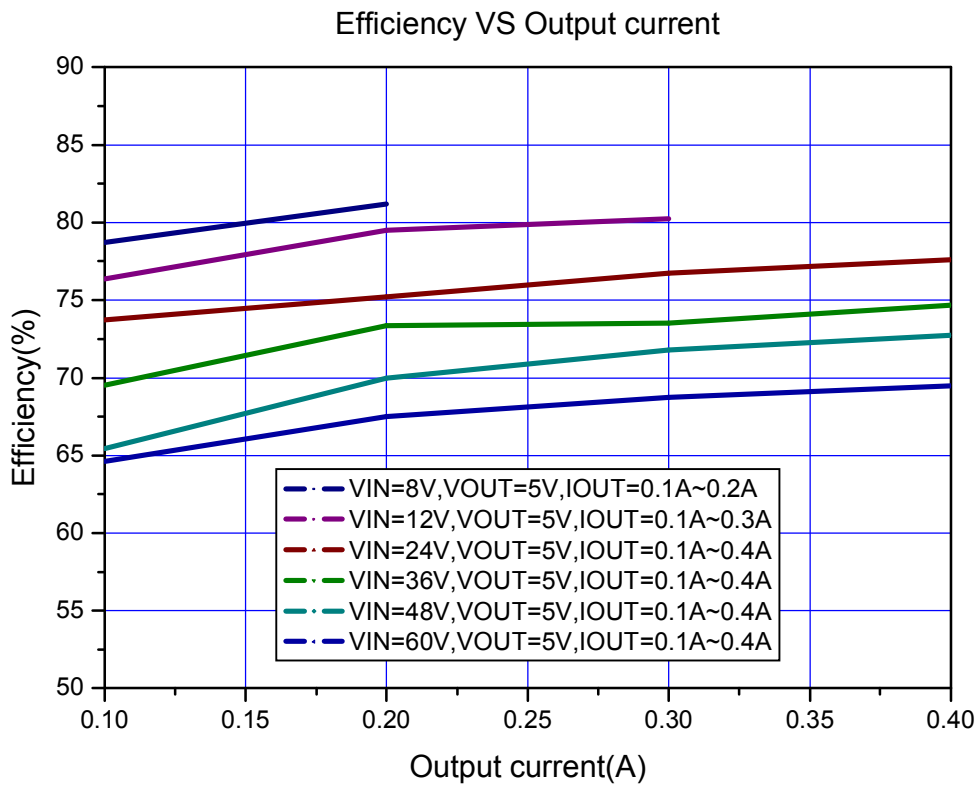
Figure8. XL7005 System Application (Efficiency VS Output Current)
