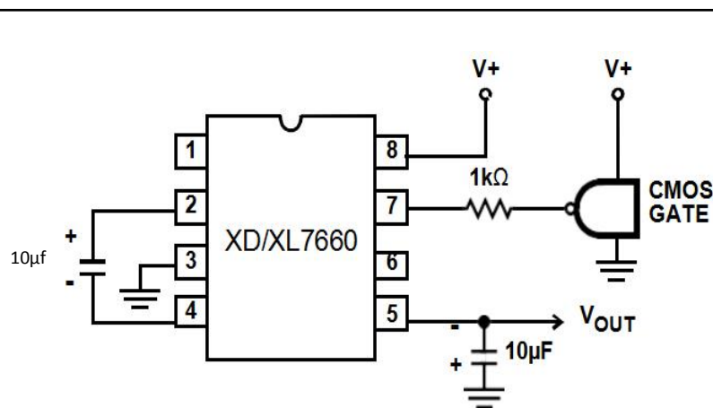
Figure 15. EXTERNAL CLOCKING
