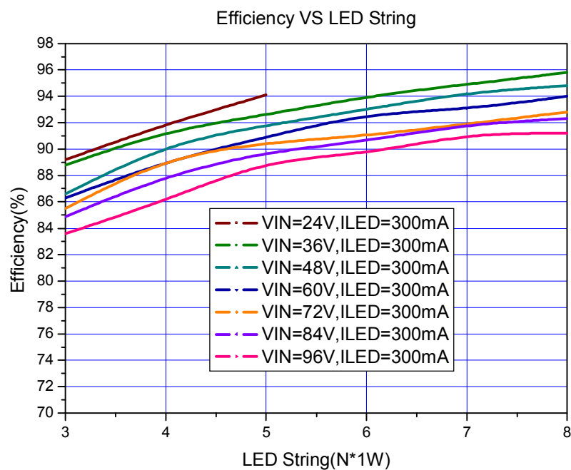
Figure5. XL8005 System Application& efficiency curve
