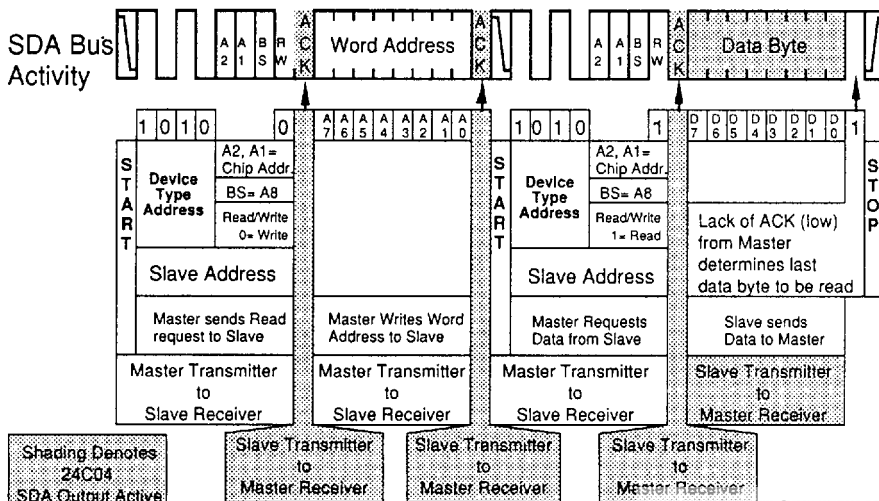
FIGURE 8. RANDOM ACCESS BYTE READ
