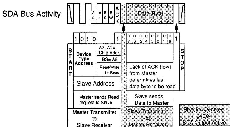
FIGURE 7. CURRENT ADDRESS BYTE READ
