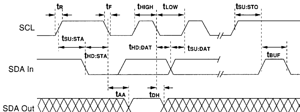
FIGURE 10. BUS TIMING
