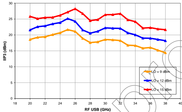
XM1004-BD: IIP3 (dBm) vs. RF USB (GHz) IF = 2 GHz at -13 dBm per Tone
