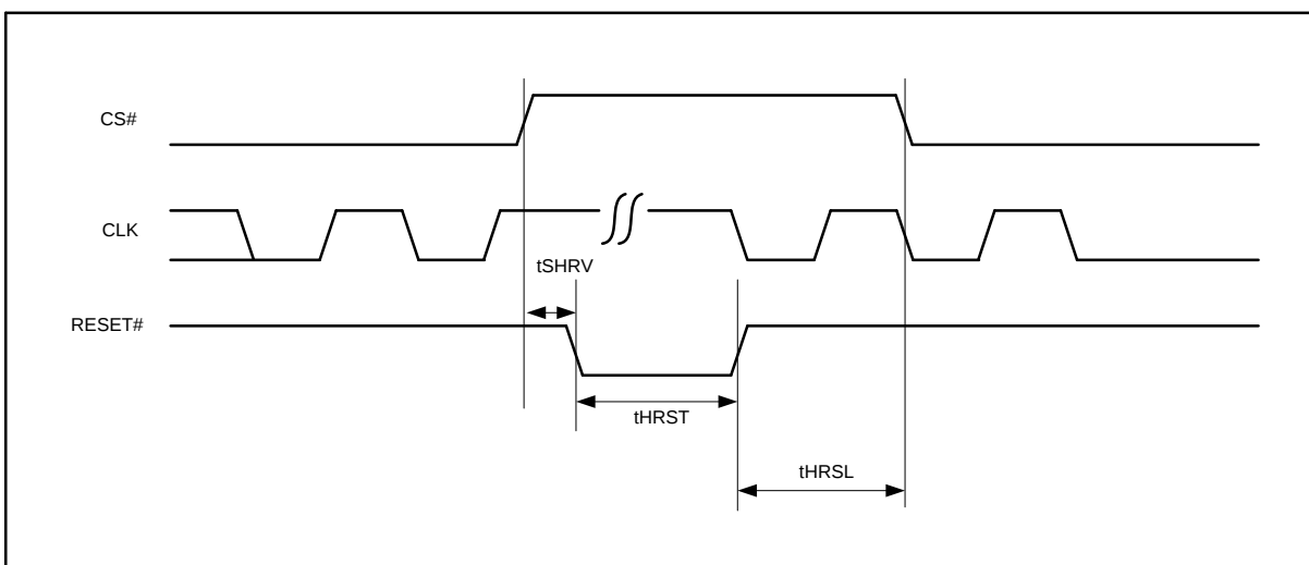
Figure 33. Reset Timing
