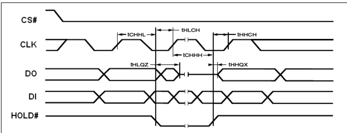
Figure 32. Hold Timing
