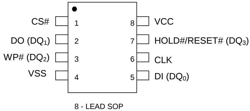
Figure.1 CONNECTION DIAGRAMS
