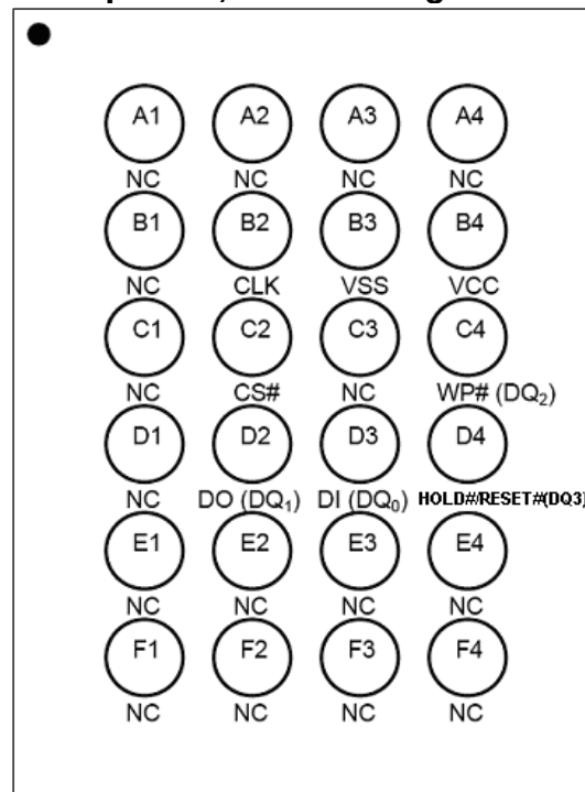
24 - Ball TFBGA
