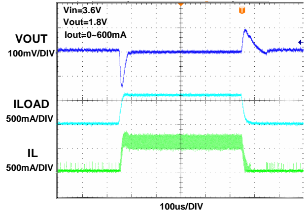
Load Transient Waveform
