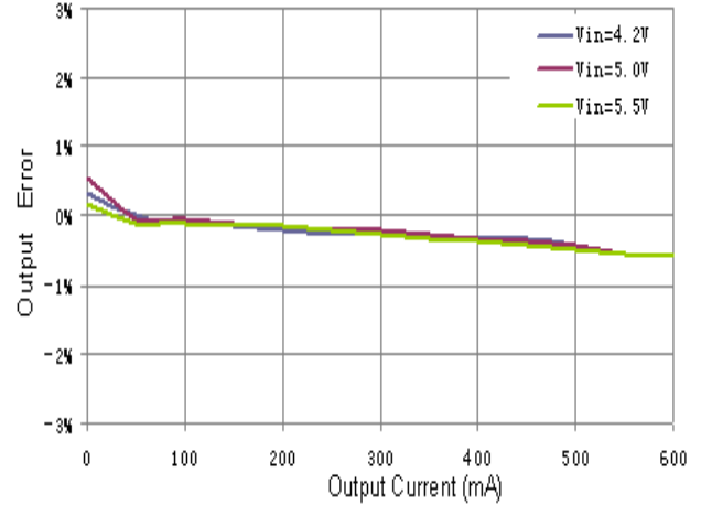
DC Regulation(Vout=3.3V)
