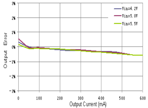
DC Regulation(Vout=3.3V)
