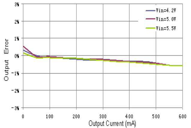
DC Regulation(Vout=1.8V)
