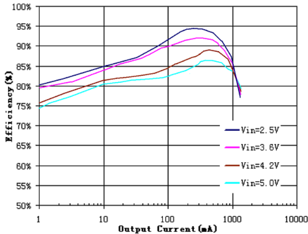
Efficiency vs. Output Current ( Vout=1.8V )
