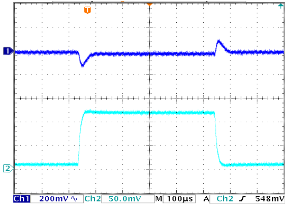
Transient Waveform(Vout=3.3V,Iout=0.15A-1.5A)
