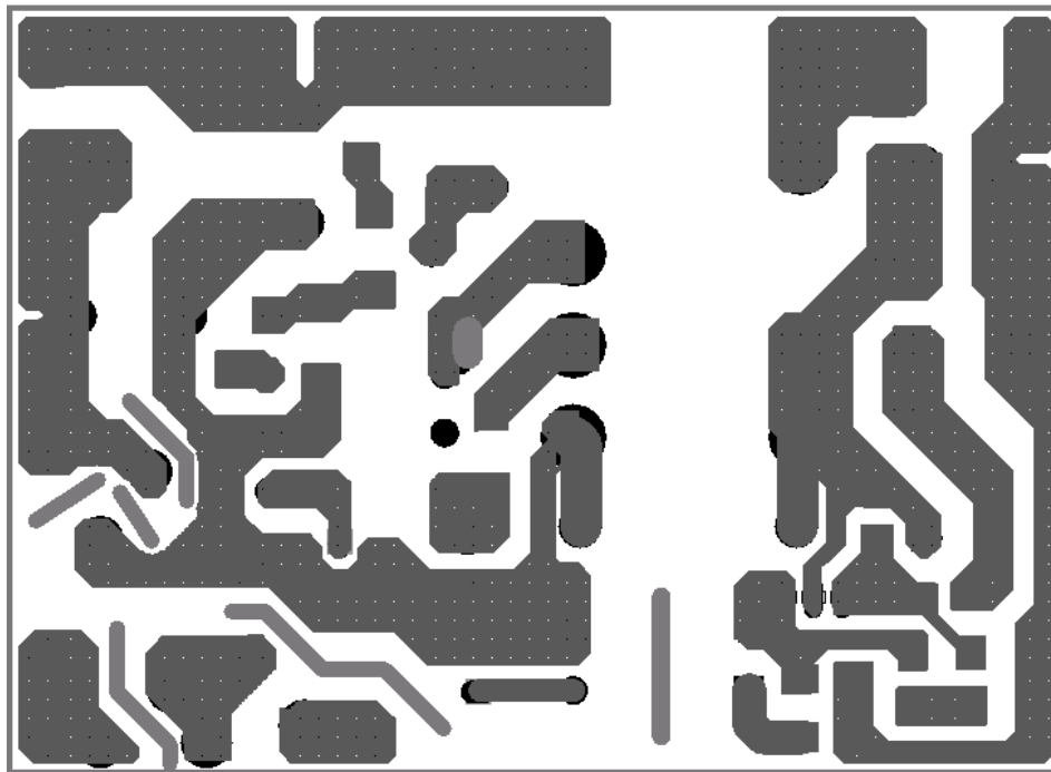
PCB Layout
