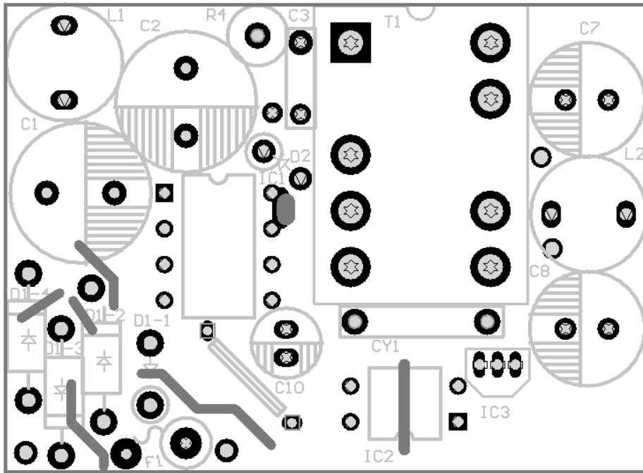
PCB Top Overlay
