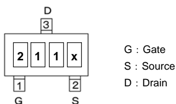
SOT-23 (TOP VIEW)
