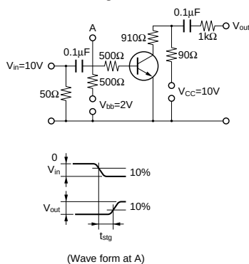
t_{stg} Test Circuit
