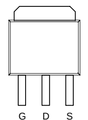
TO-251VS(JV)
