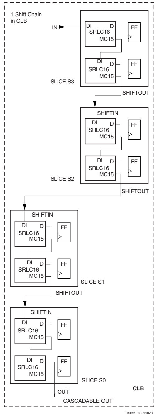
Figure 23: Cascadable Shift Register
