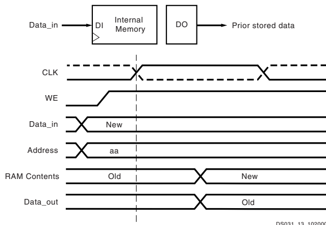
Figure 33: READ_FIRST Mode
