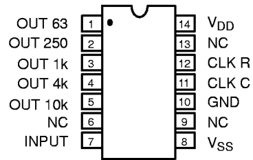
14 Lead PDIP (0.300")
