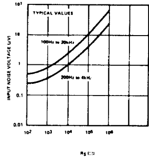
BROADBAND INPUT NOISE VOLTAGE
