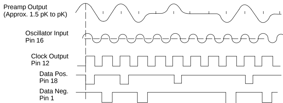
Figure 4. Typical T56L22 Waveforms
