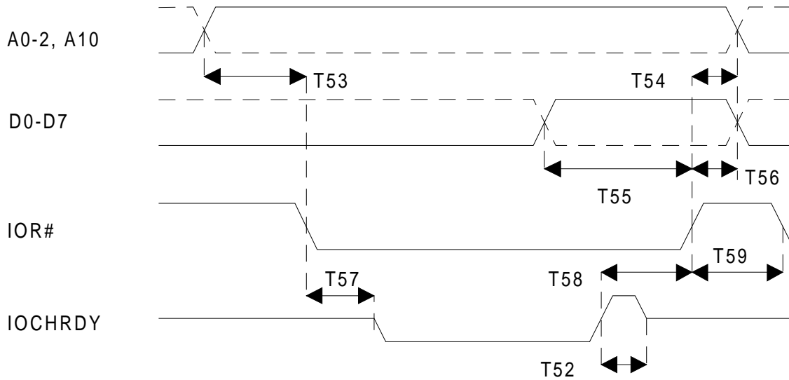
Address or data read timing in EPP mode
