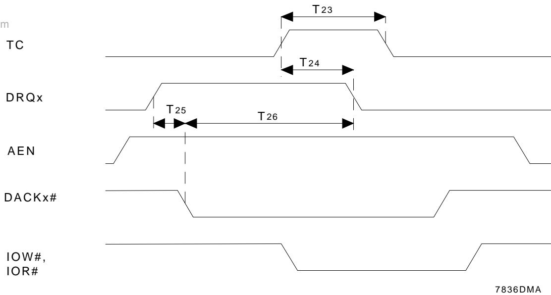
Host DMA timing in ECP mode
