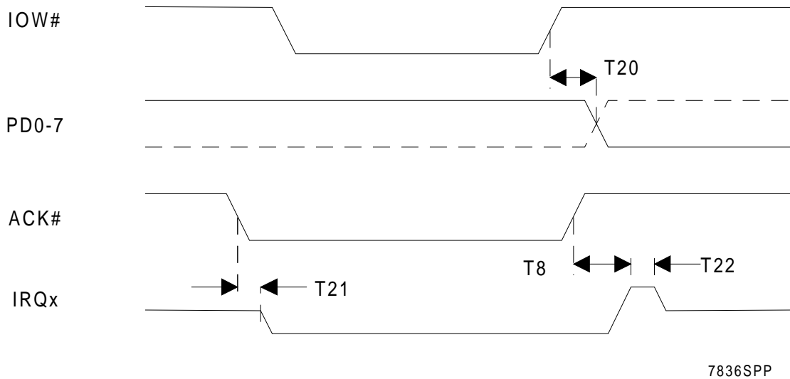
Parallel port timing in SPP, PS/2 mode
