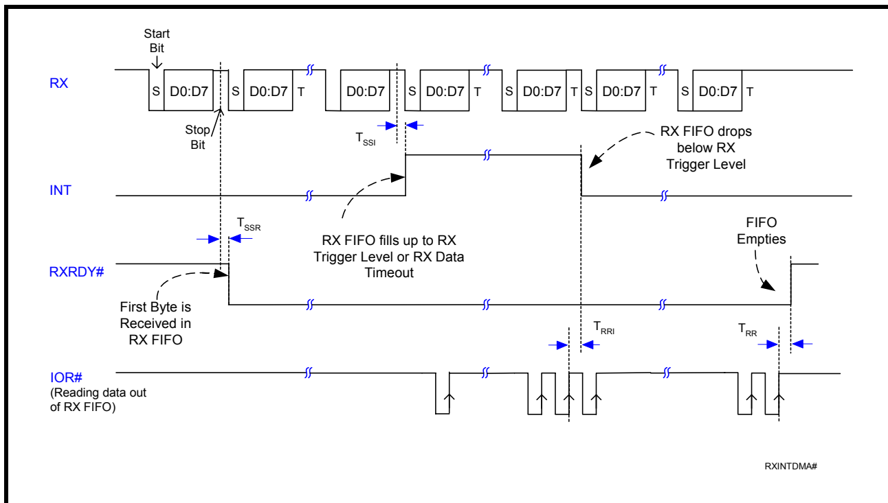
FIGURE 21. RECEIVE READY & INTERRUPT TIMING [FIFO MODE, DMA DISABLED] FOR CHANNELS A & B
