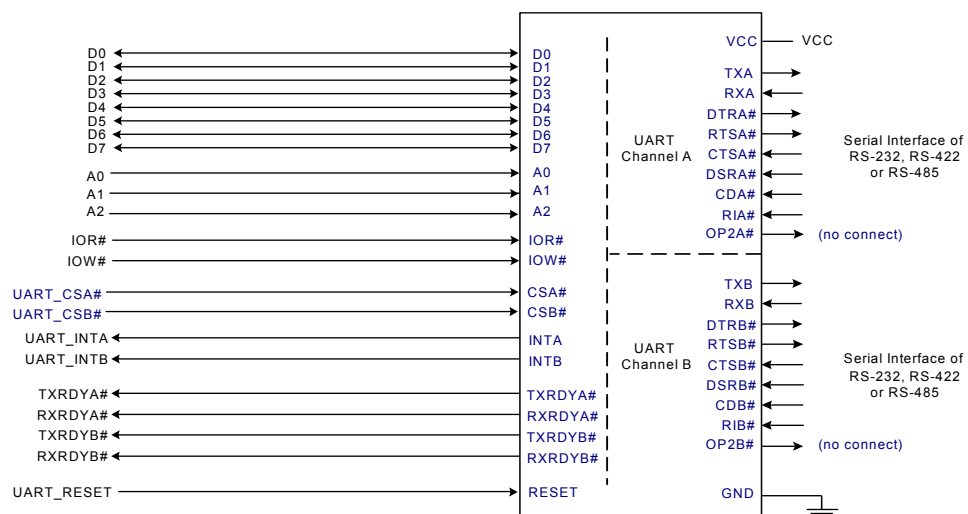
FIGURE 3. XR16M752/XR68M752 DATA BUS INTERCONNECTIONS
