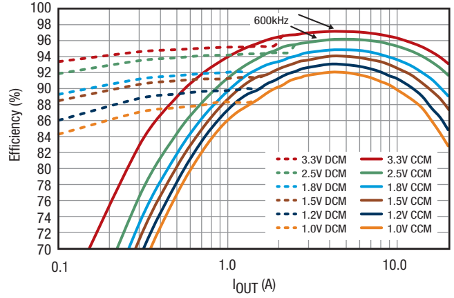
Figure 4. XR76120 Efficiency, V_{IN} = 5V, L = 0.4\mu H
