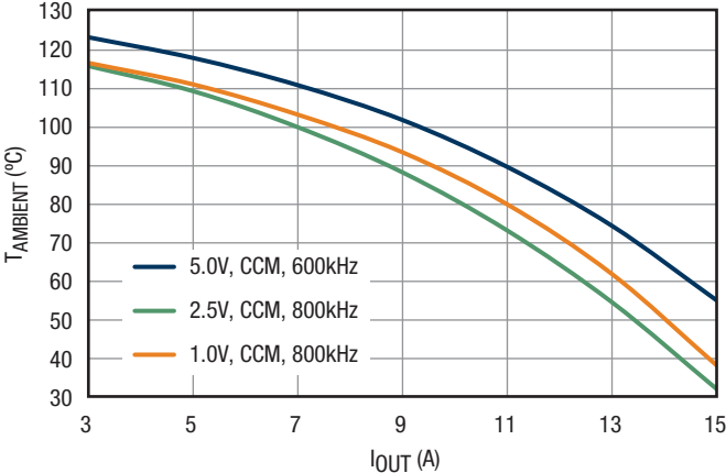
Figure 9. XR76116 Maximum T_{AMBIENT} vs. I_{OUT} , V_{IN} = 12V , No Airflow
