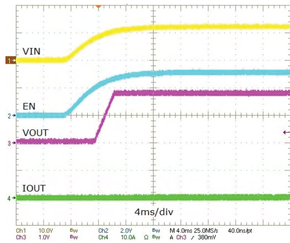
Figure 10. Power-Up, I_{OUT} = 0A
