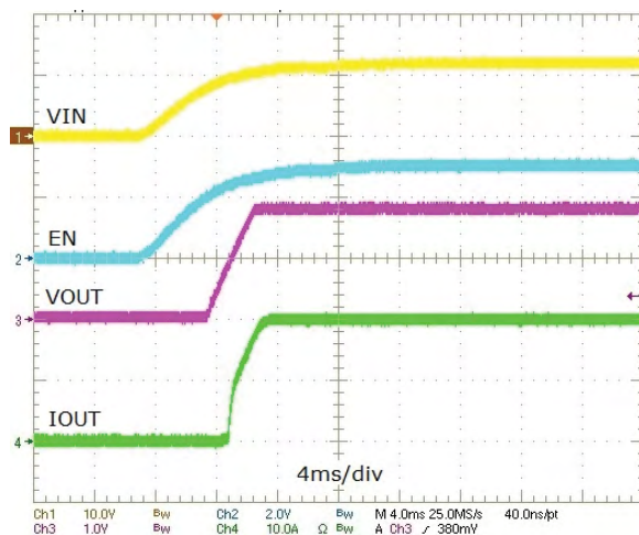
Figure 9. Power-Up, I_{OUT} = 20A
