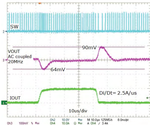
Figure 11. Load Transient, Forced CCM, 0A-10A-0A
