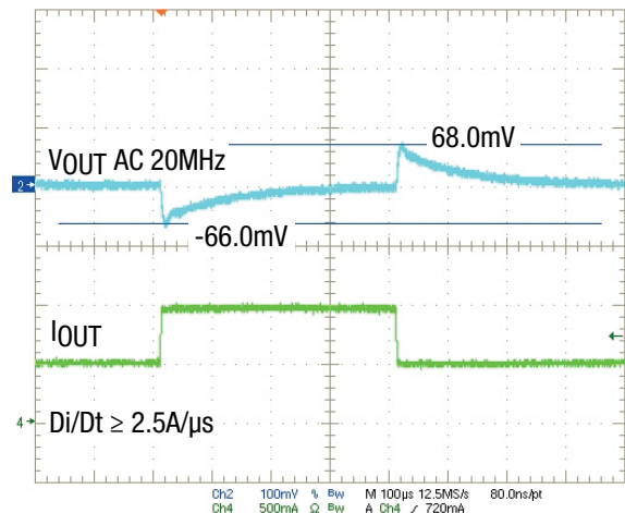
Figure 13. 5\text{V}_{\text{IN}} , 1.8\text{V}_{\text{OUT}} Transient Response, 0.5\text{A} to 1.0\text{A}
