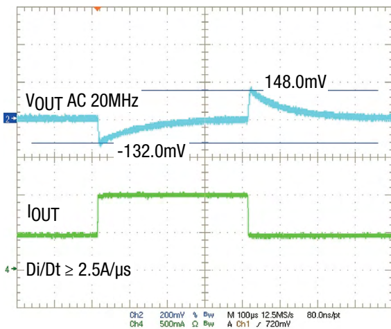
Figure 10. 12\text{V}_{\text{IN}} , 3.3\text{V}_{\text{OUT}} Transient Response, 0.5\text{A} to 1.0\text{A}
