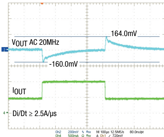
Figure 12. 5\text{V}_{\text{IN}} , 3.3\text{V}_{\text{OUT}} Transient Response, 0.5\text{A} to 1.0\text{A}
