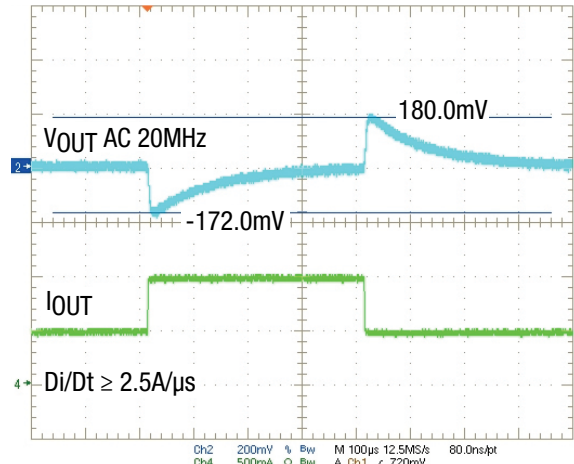
Figure 9. 12\text{V}_{\text{IN}} , 5.0\text{V}_{\text{OUT}} Transient Response, 0.5\text{A} to 1.0\text{A}
