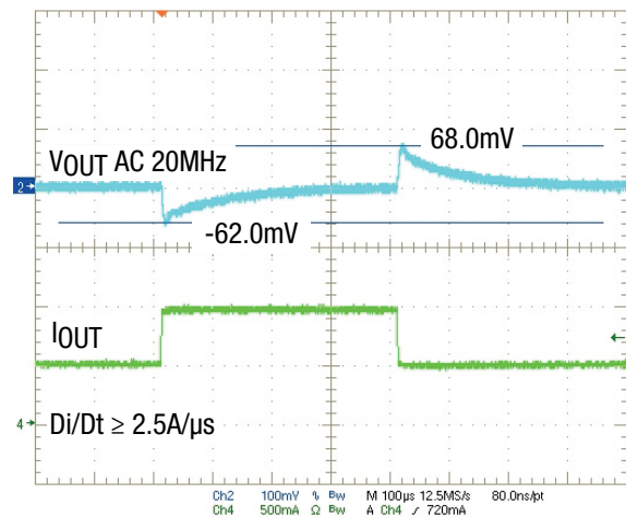
Figure 11. 12\text{V}_{\text{IN}} , 1.8\text{V}_{\text{OUT}} Transient Response, 0.5\text{A} to 1.0\text{A}
