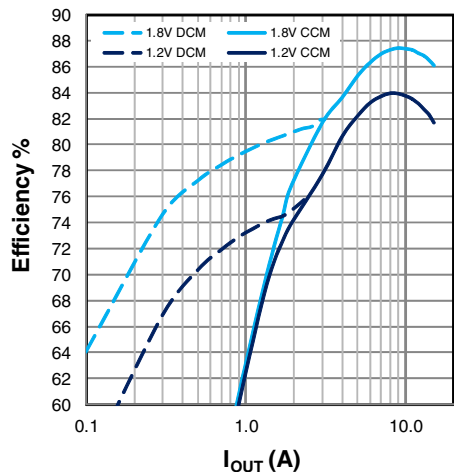
Figure 23: Efficiency, V_{IN}=19.6V
