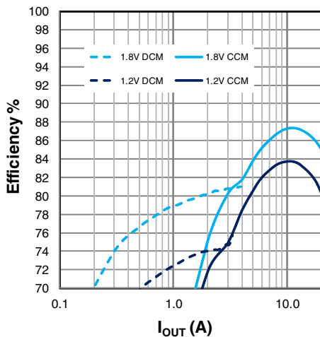
Figure 23: Efficiency, V_{IN}=19.6\text{V}
