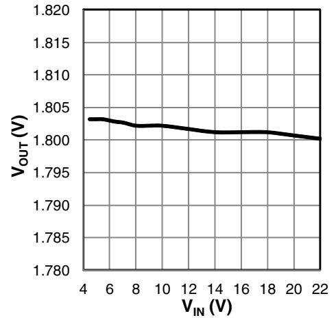
Figure 2: Line regulation
