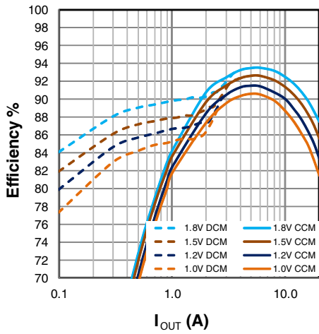
Figure 19: Efficiency, V_{IN}=5\text{V}
