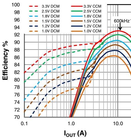
Figure 21: Efficiency, V_{IN}=12\text{V}
