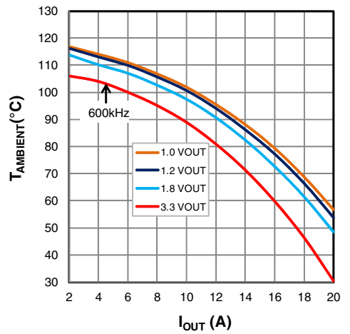
Figure 22: Maximum T_{AMBIENT} vs I_{OUT} , V_{IN}=12\text{V}
