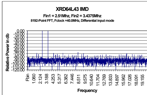
Figure 10. Intermodulation Distortion, Fin1=2.51MHz, Fin2=3.4375MHz, 8192-point FFT, Fc=40MHz, Differential Input Mode
