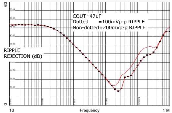
Fig. 12: PSRR, 50mA, 1.5VIN, 1VOUT, 47uF C OUT
