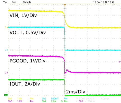
Fig. 10: Powerdown, IO UT =3A, 1.5VIN, 1VOUT
