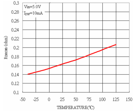
Fig. 11: NMOS R_{DS(ON)} vs Temperature
