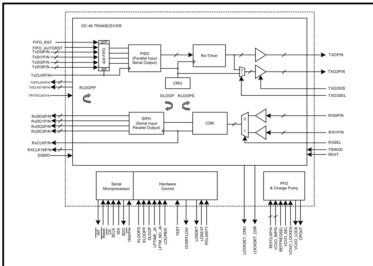
FIGURE 1. BLOCK DIAGRAM OF THE XRT91L81
