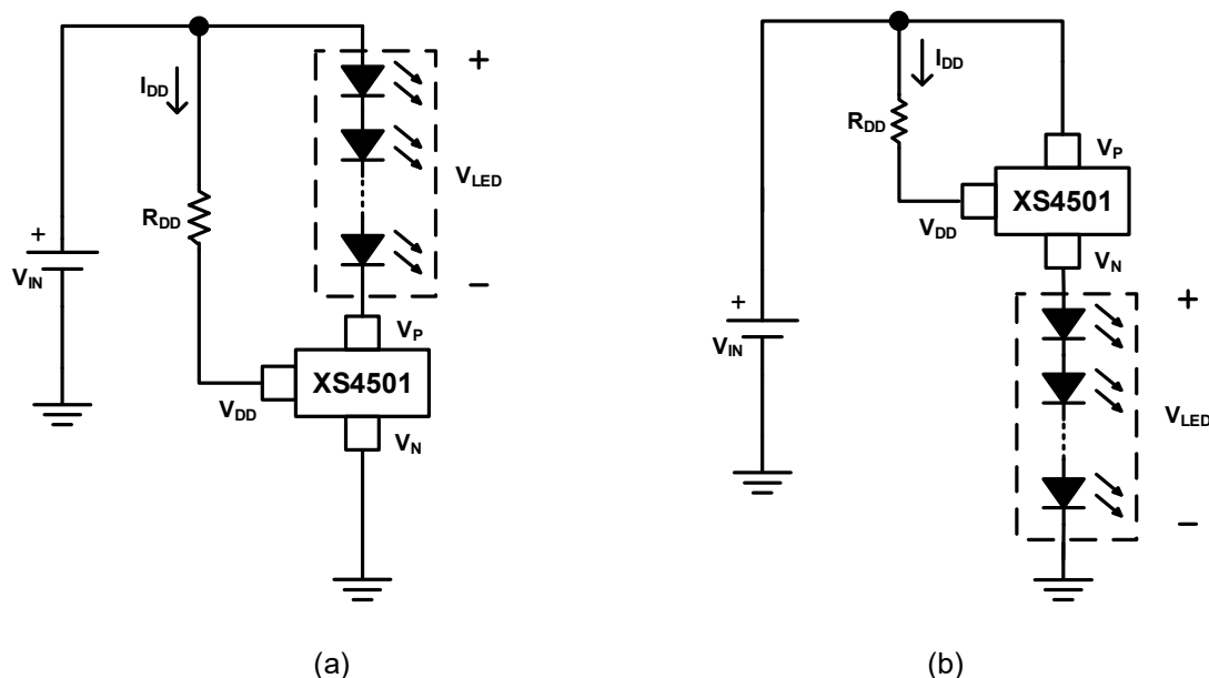
Figure 7. (a) Low-side LED Driver (b) High-side LED Driver
