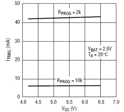
Trickle Charge Current vs Supply Voltage
