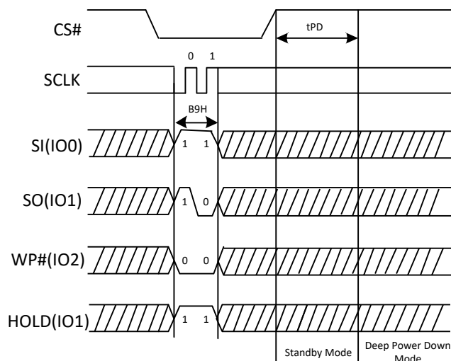
Figure 21a. Deep Power-Down Sequence Diagram (QPI)
