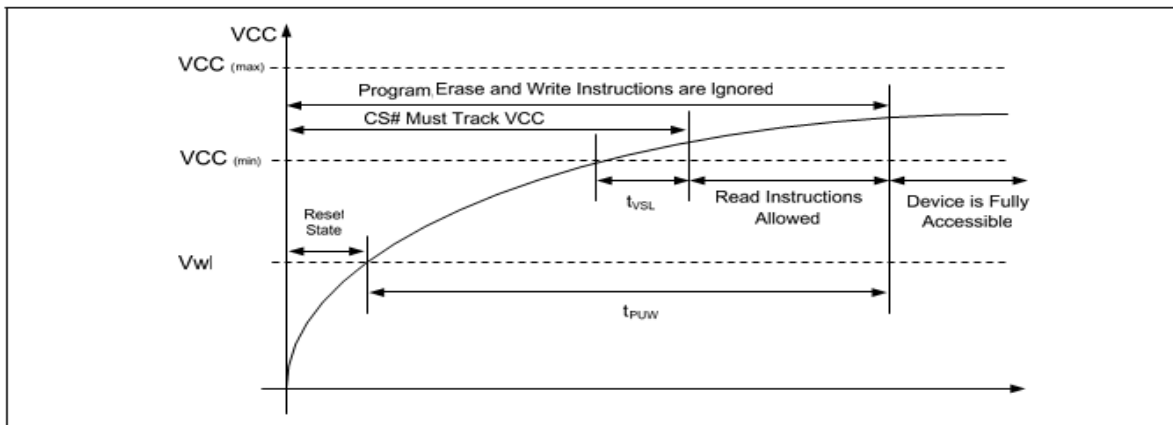
Figure 32 Power-On Timing
