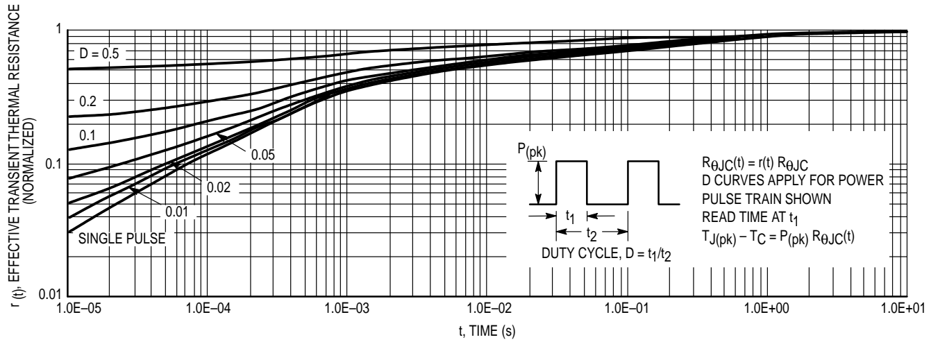
Figure 13. Thermal Response
