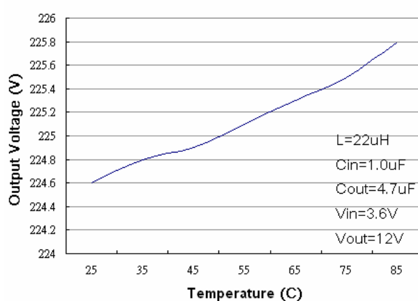
VFB Voltage vs Temperature
