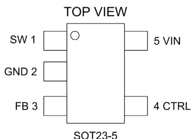
Figure 3 : YB1517 Pin Configuration
