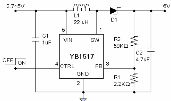
Figure 5 : TFT Panel Power Application Circuit
