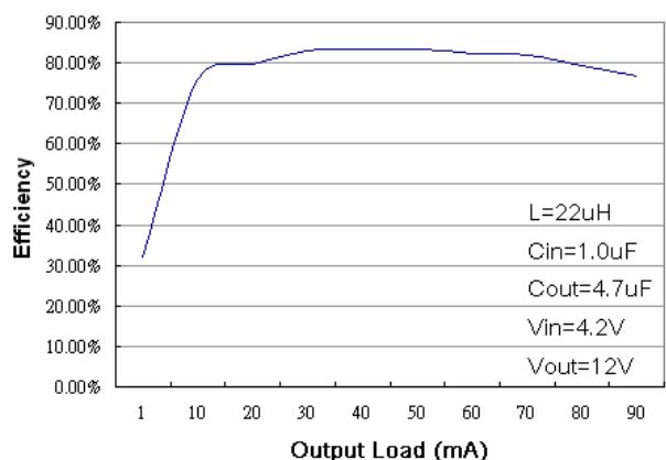
Efficiency vs Output Load (2)
