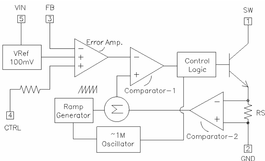
Figure 3: YB1517 Block Diagram
