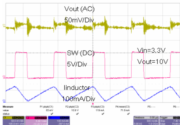
Output Waveform at 20 mA Load (2)
