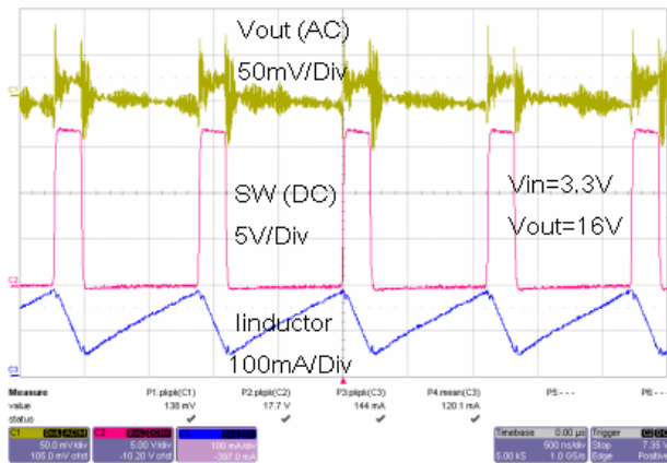
Output Waveform at 20 mA Load (1)
