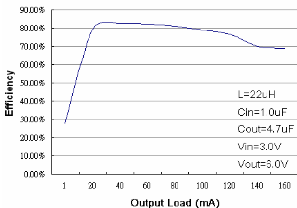
Efficiency vs Output Load (3)
