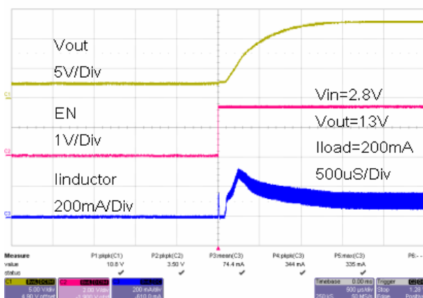
Soft-Start Waveform
