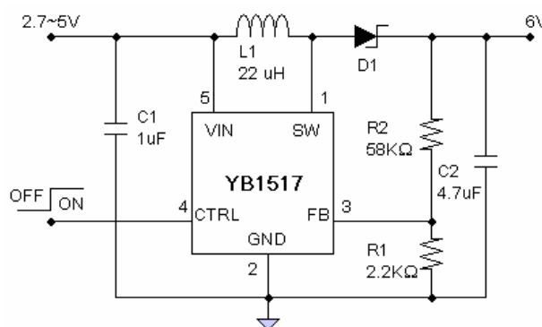
Figure 2 : DC-to-DC Converter
