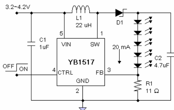
Figure 1 : White LED Driver
