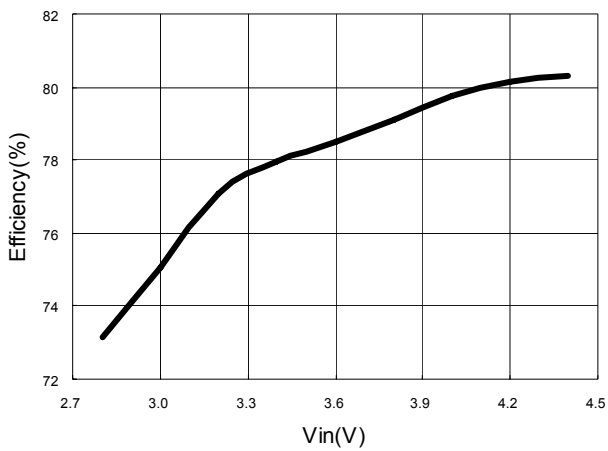
Efficiency vs Vin (6WLEDs)
