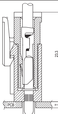
PCB ASSY
