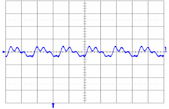
Fig. 2.0V.5: Output voltage ripple (20mV/div.) at full rated load current into a resistive load with external capacitance 100\ \mu\text{F} ceramic + 1\ \mu\text{F} ceramic and V_{in} = 12\text{ V} for V_{out} = 2.0\text{ V} . Time scale: 2 \mu\text{s} /div.
