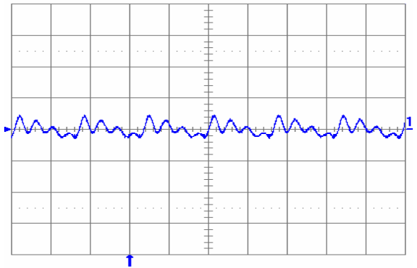
Fig. 1.2V.5: Output voltage ripple (20 mV/div.) at full rated load current into a resistive load with external capacitance 100\ \mu\text{F} ceramic + 1\ \mu\text{F} ceramic and V_{in} = 12\text{ V} for V_{out} = 1.2\text{ V} . Time scale: 2 \mu\text{s} /div.
