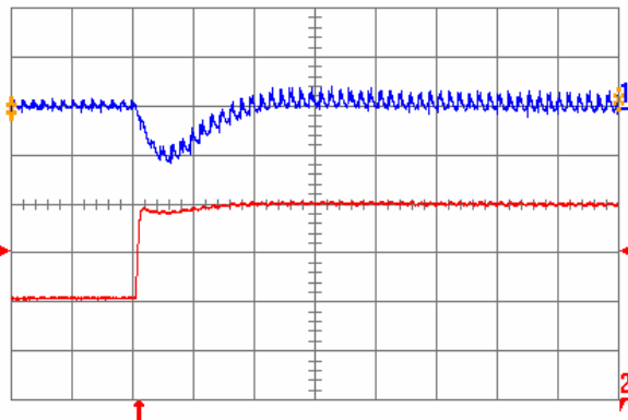
Fig. 2.5V.6: Output voltage response for V_{out} = 2.5\text{ V} to positive load current step change from 10 A to 20 A with slew rate of 5\text{A}/\mu\text{s} at V_{in} = 12\text{ V} . Top trace: output voltage (200 mV/div.); Bottom trace: load current (5 A/div.). C_o = 100\ \mu\text{F} ceramic. Time scale: 20 \mu\text{s} /div.
