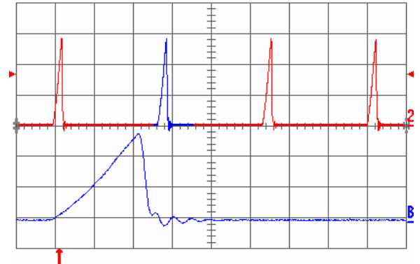
Fig. D: Output short circuit current (10 A/div) ( R_{LOAD} = 10 mOhm) for V_{out} = 5.0 V Time scale: 1 ms/div.; Bottom trace: Zoomed current with time scale 0.1 ms/div.
