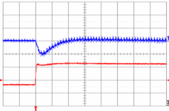
Fig. 2.0V.6: Output voltage response for V_{out} = 2.0\text{ V} to positive load current step change from 10 A to 20 A with slew rate of 5\text{ A}/\mu\text{s} at V_{in} = 12\text{ V} . Top trace: output voltage (200 mV/div.); Bottom trace: load current (5 A/div.). C_o = 100\ \mu\text{F} ceramic. Time scale: 20 \mu\text{s} /div.
