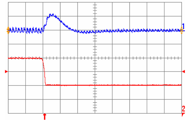
Fig. 3.3V.7: Output voltage response for V_{out} = 3.3\text{ V} to negative load current step change from 20 A to 10 A with slew rate of -5\text{ A}/\mu\text{s} at V_{in} = 12\text{ V} . Top trace: output voltage (200 mV/div.); Bottom trace: load current (5 A/div.). C_o = 100\ \mu\text{F} ceramic. Time scale: 20 \mu\text{s} /div.
