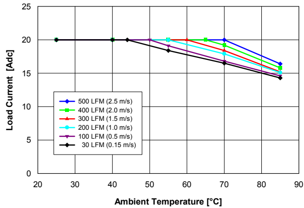
Fig. 1.0V.1: Available load current vs. ambient temperature and airflow rates for V out = 1.0 V converter mounted vertically with V in = 12 V, and maximum MOSFET temperature ≤ 120 °C.
