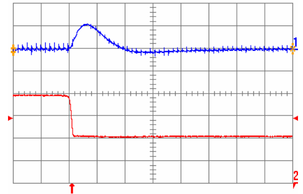
Fig. 0.7525V.7: Output voltage response for V_{out} = 0.7525 V to negative load current step change from 20 A to 10 A with slew rate of -5\text{A}/\mu\text{s} at V_{in} = 12 V. Top trace: output voltage (200 mV/div.); Bottom trace: load current (5 A/div.). C_o = 100 \mu\text{F} ceramic. Time scale: 20 \mu\text{s} /div.
