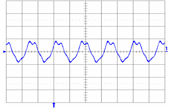
Fig. 5.0V.5: Output voltage ripple (20 mV/div.) at full rated load current into a resistive load with external capacitance 100\ \mu\text{F} ceramic + 1\ \mu\text{F} ceramic and V_{in} = 12\text{ V} for V_{out} = 5.0\text{ V} . Time scale: 2 \mu\text{s} /div.
