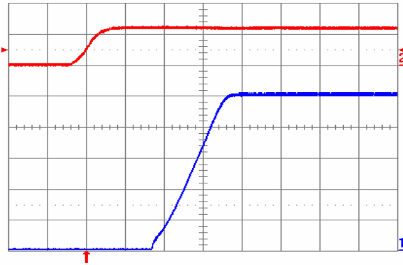
Fig. 5.0V.4: Turn-on transient for V_{out} = 5.0\text{ V} with application of V_{in} at full rated load current (resistive) and 100\ \mu\text{F} external capacitance at V_{in} = 12\text{ V} . Top trace: V_{in} (10 V/div.); Bottom trace: output voltage (1 V/div.); Time scale: 2 ms/div.
