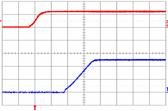
Fig. 2.5V.4: Turn-on transient for V_{out} = 2.5\text{ V} with application of V_{in} at full rated load current (resistive) and 100\ \mu\text{F} external capacitance at V_{in} = 12\text{V} . Top trace: V_{in} (10 V/div.); Bottom trace: output voltage (1 V/div.); Time scale: 2 ms/div.
