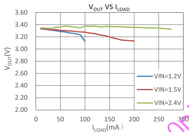
图 1. V_{OUT} VS I_{LOAD} (L=22uH)
