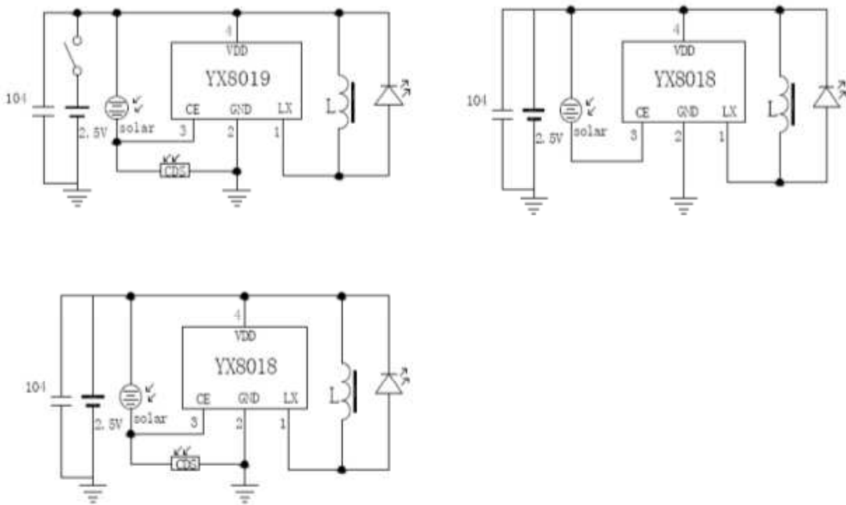
Application 2 (1.25V rechargeable battery x2 pieces)
