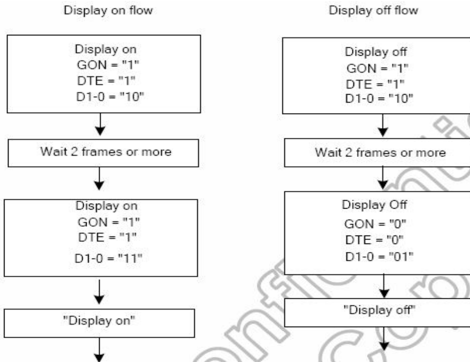
Figure 5.37: Display on/off set flow
